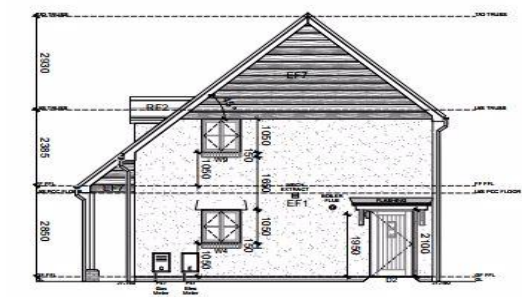
4 PLOT 47 & 48 - SIDE ELEVATION (SOUTH) Scale: 1:50
